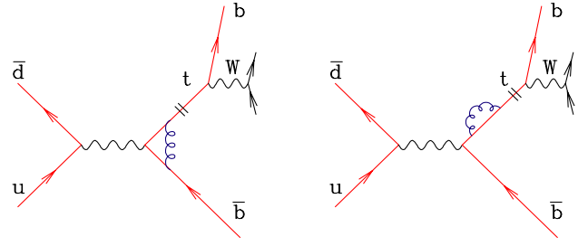
FIG. 5 (color online). Final-state virtual radiation in the production stage.
