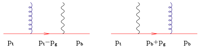
FIG. 10 (color online). Real radiation in free top decay.
