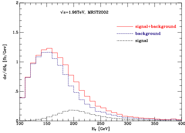
FIG. 12 (color online). The H_T distributions of signal, background, and signal plus background. The curves correspond to the sum of the appropriate distributions shown in Fig. 11.
